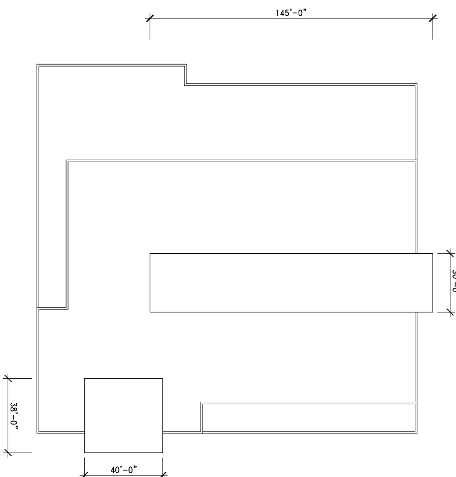
Roof Plan
