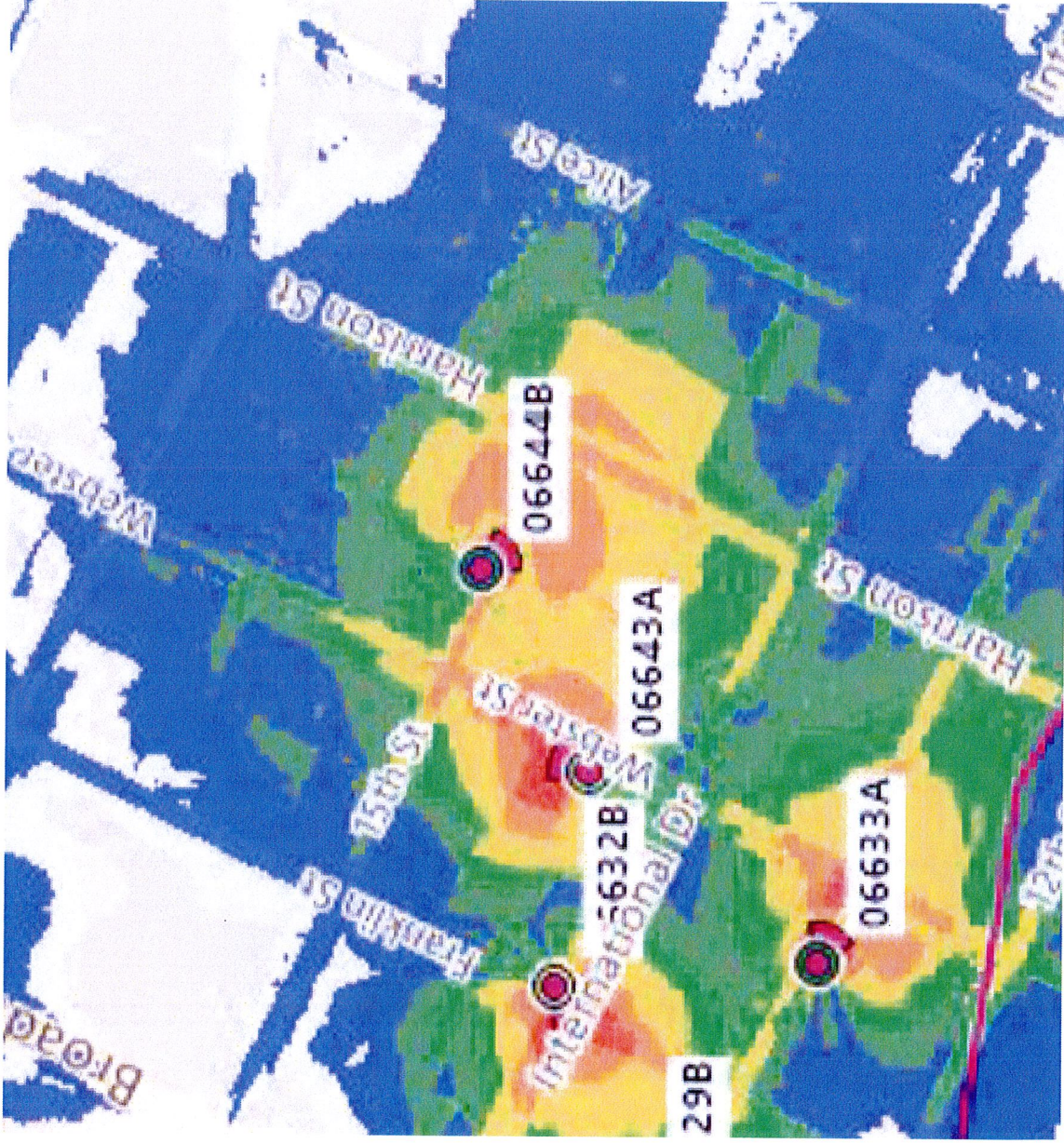
This propagation map depicts the ExteNet proposed Node 06644B in relation to surrounding proposed ExteNet small cell nodes.
