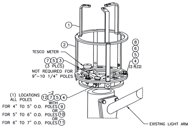
CLAMP-ON BRACKET
