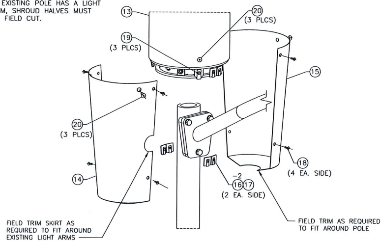
SHROUD ASSEMBLY
