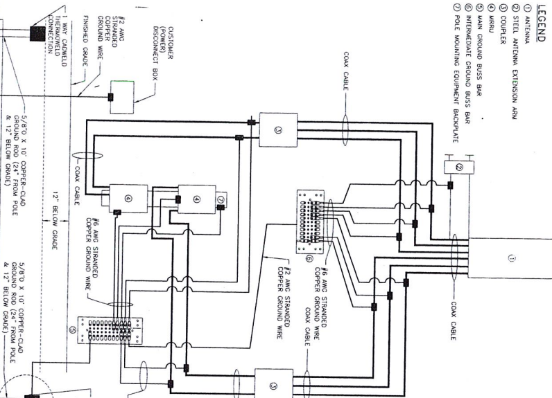
CONCEPTUAL WOOD POLE GROUNDING DETAIL
