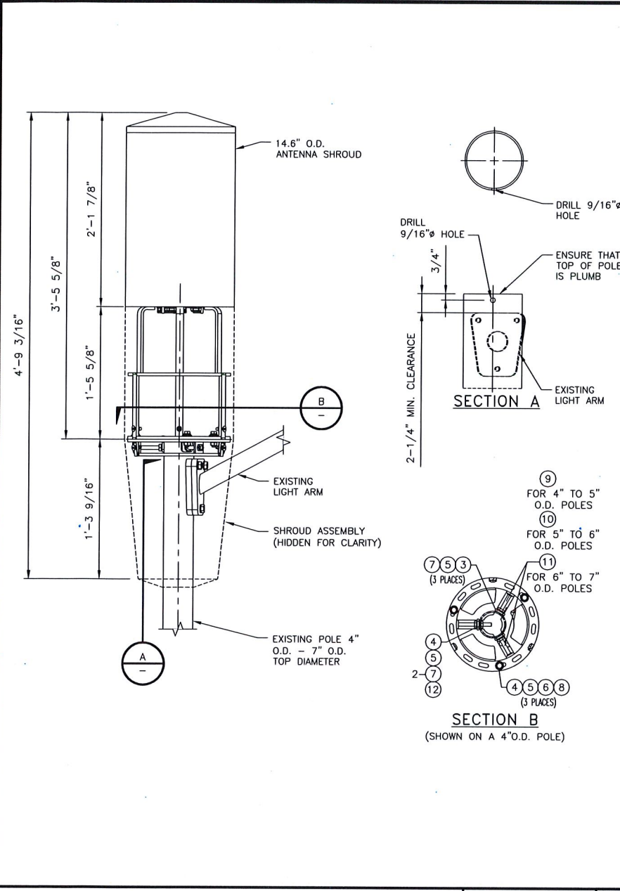
SHROUD/ANTENNA ELEVATION VIEW NO SCALE 1
