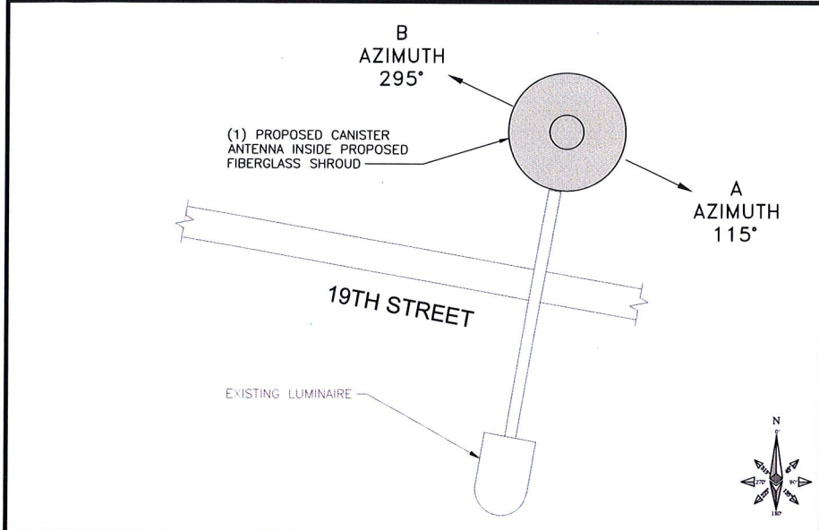
ANTENNA SPACE PLAN VIEW NO SCALE 1
