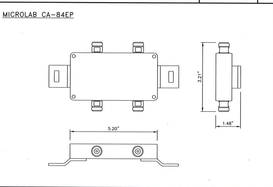
DIPLEXER SPECIFICATIONS NO SCALE 8
