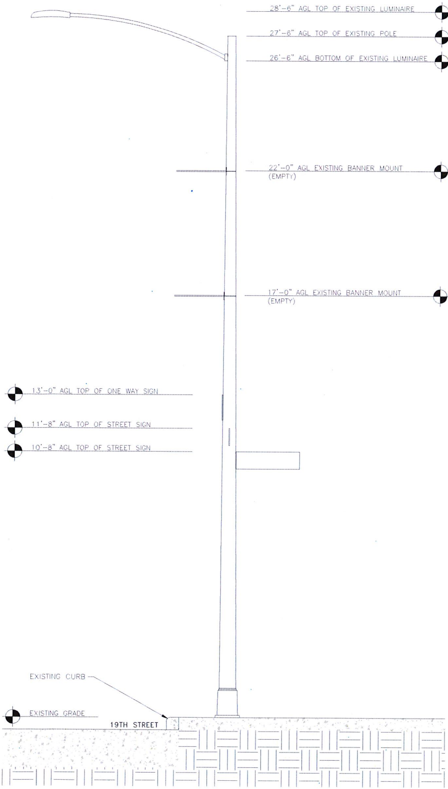
EXISTING EAST ELEVATION
