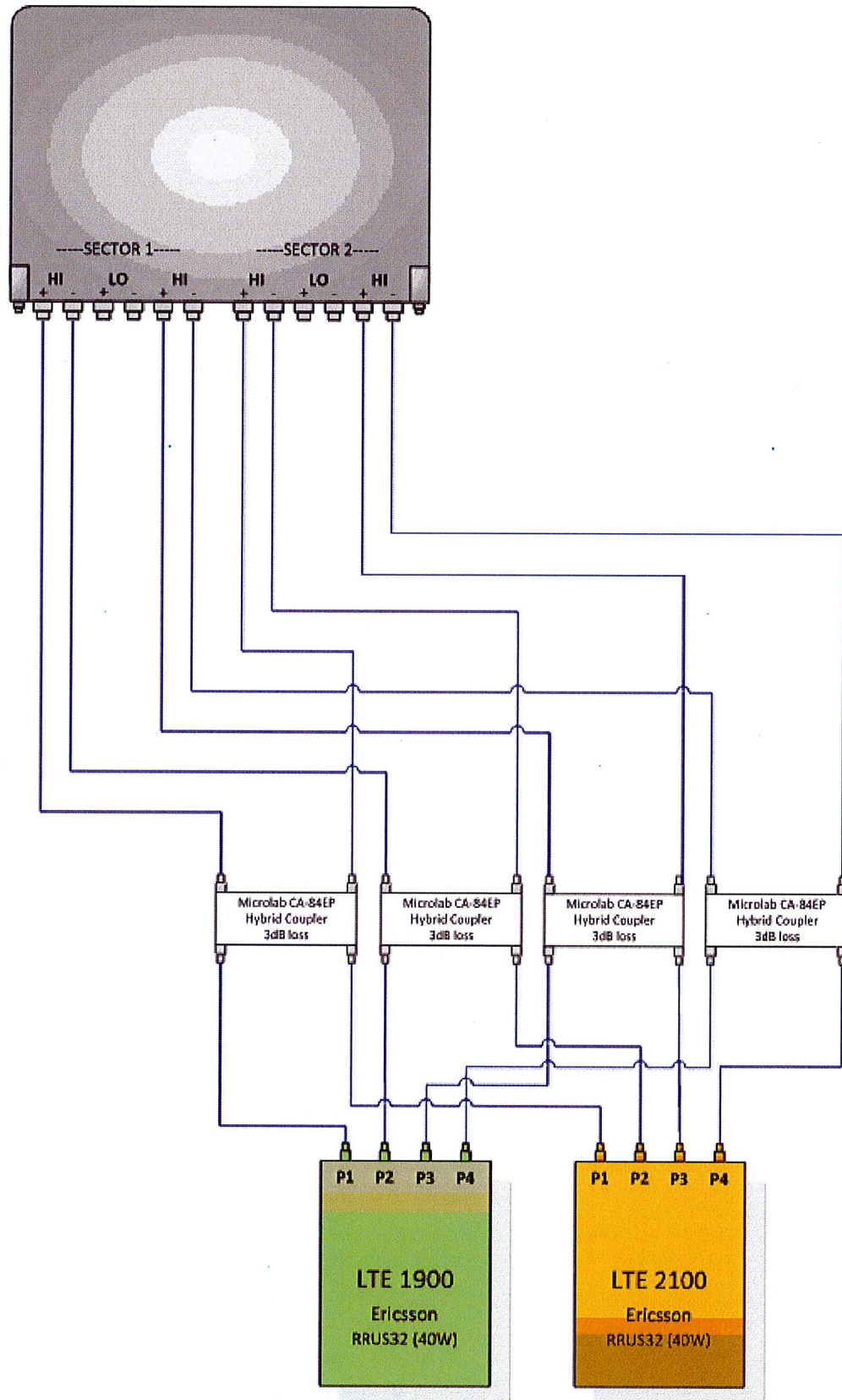
ANTENNA CONFIGURATION
