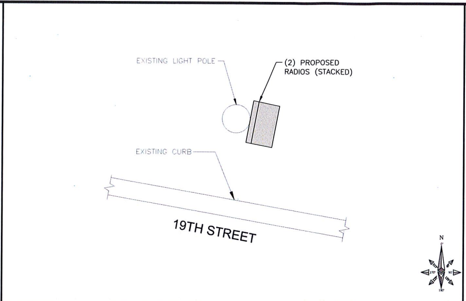
RADIO SPACE PLAN VIEW NO SCALE 2
