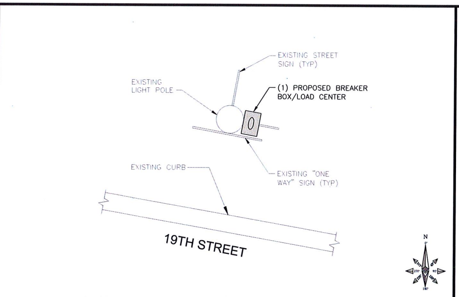
EQUIPMENT PLAN VIEW NO SCALE 3
