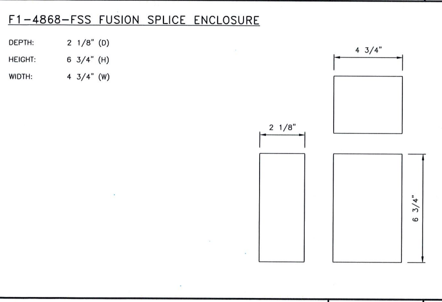
FIBER SPLICE BOX SPECIFICATIONS NO SCALE 6
