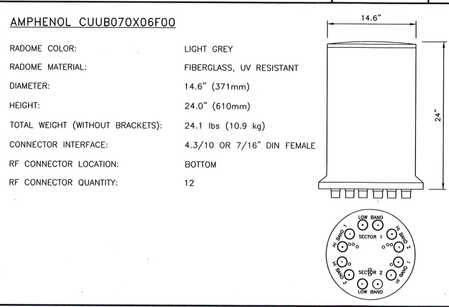
ANTENNA SPECIFICATIONS NO SCALE 7
