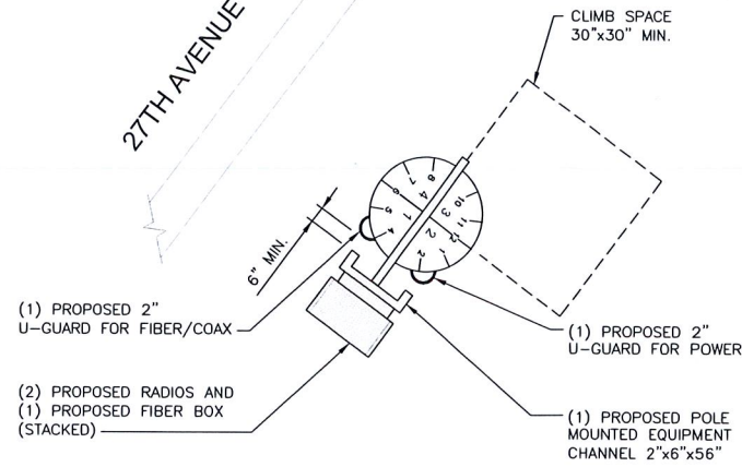
RADIO PLAN VIEW
