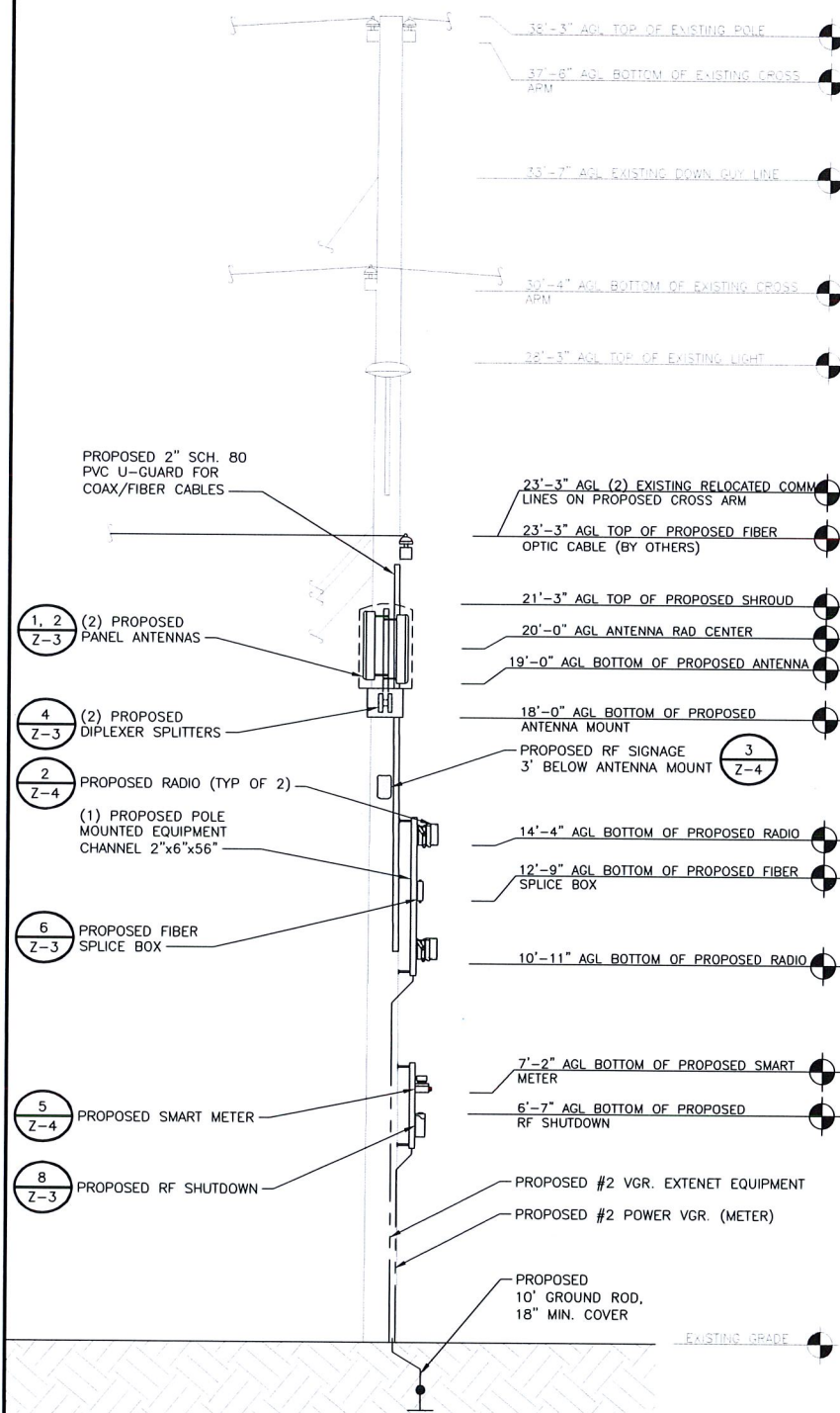
PROPOSED NORTHWEST ELEVATION
