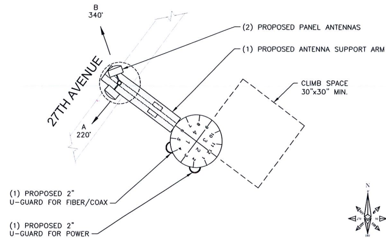
ANTENNA PLAN VIEW
