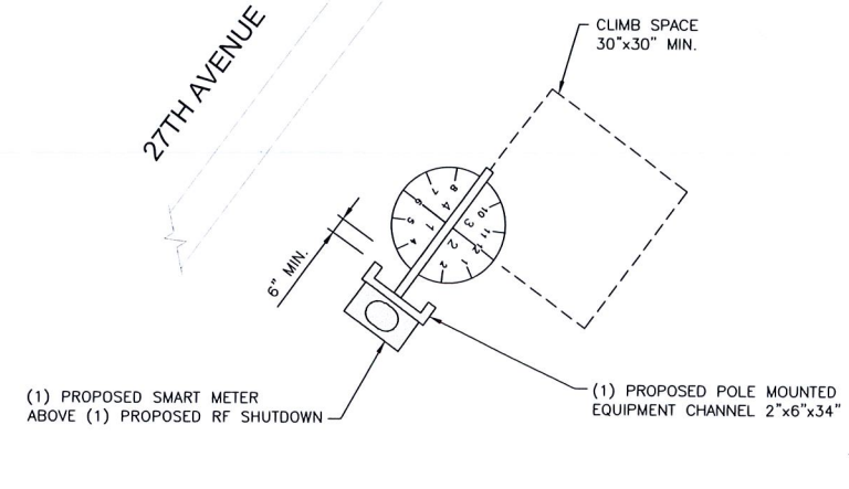
EQUIPMENT PLAN VIEW
