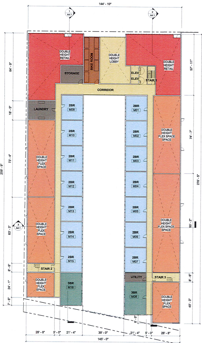
2 BLDG 1 - MEZZANINE 1/16" = 1'-0"
