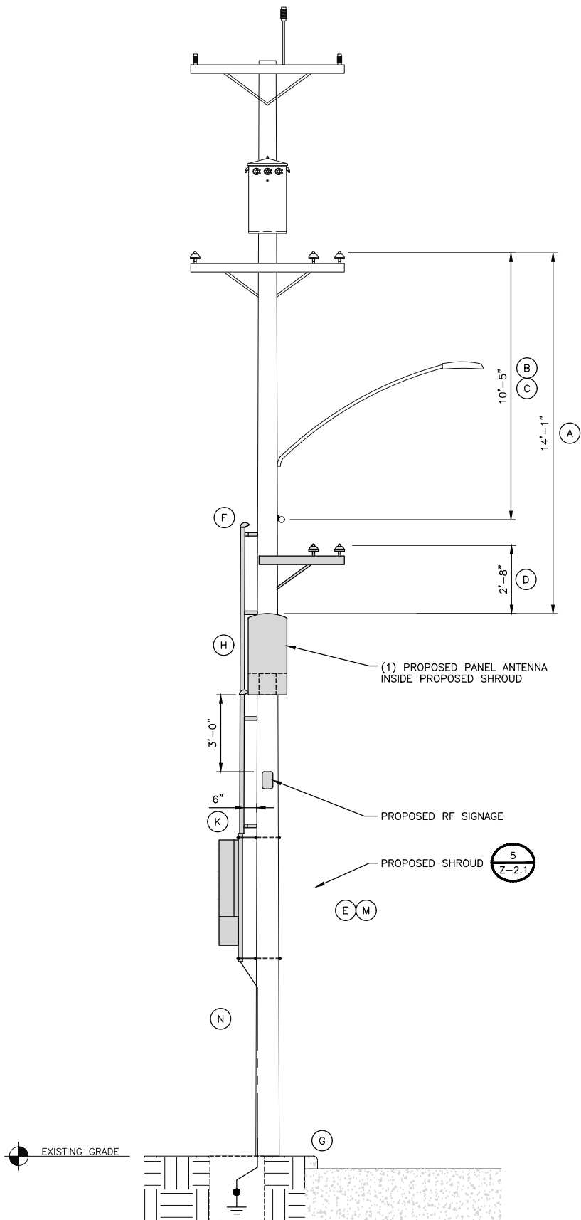
EQUIPMENT CLEARANCES
