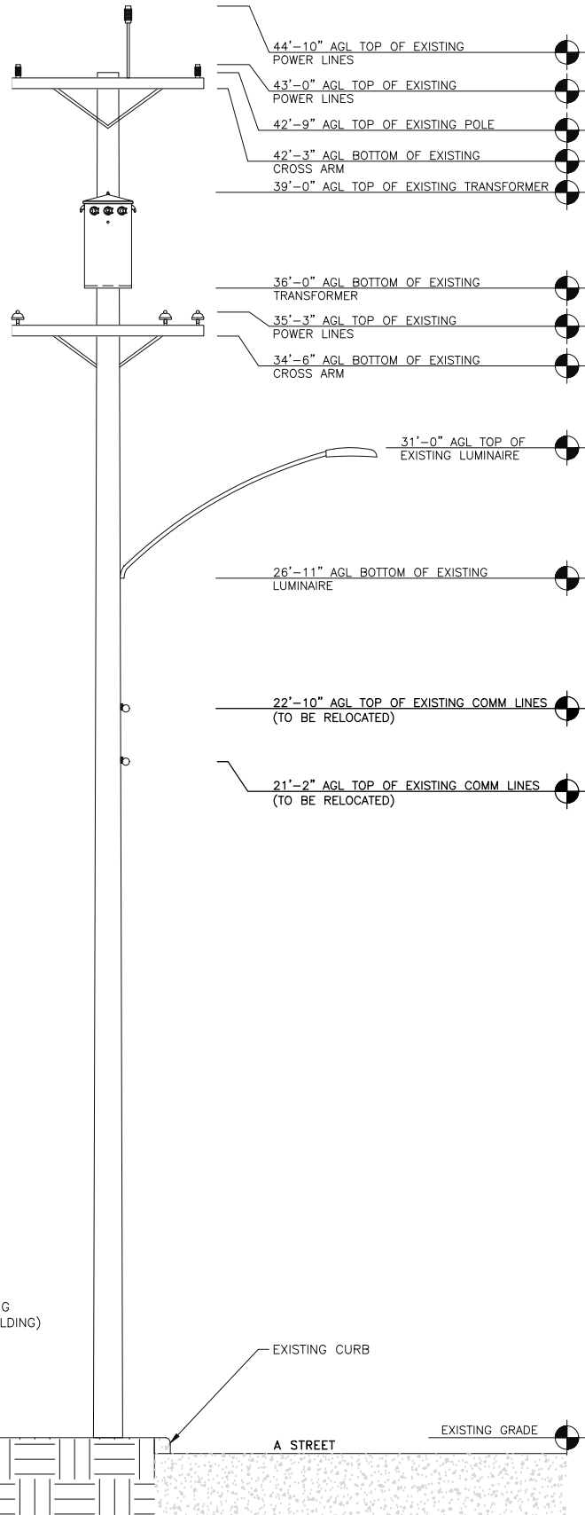
EXISTING SOUTHEAST ELEVATION
