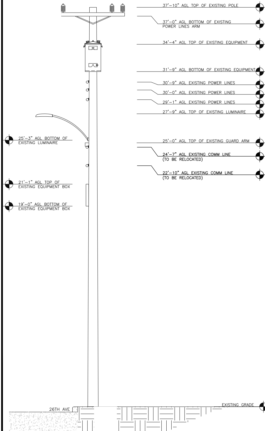
EXISTING NORTHWEST ELEVATION
