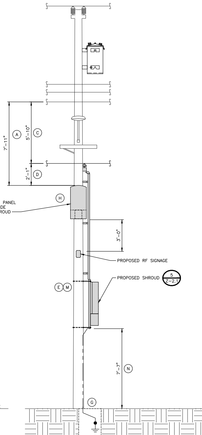
EQUIPMENT CLEARANCES
