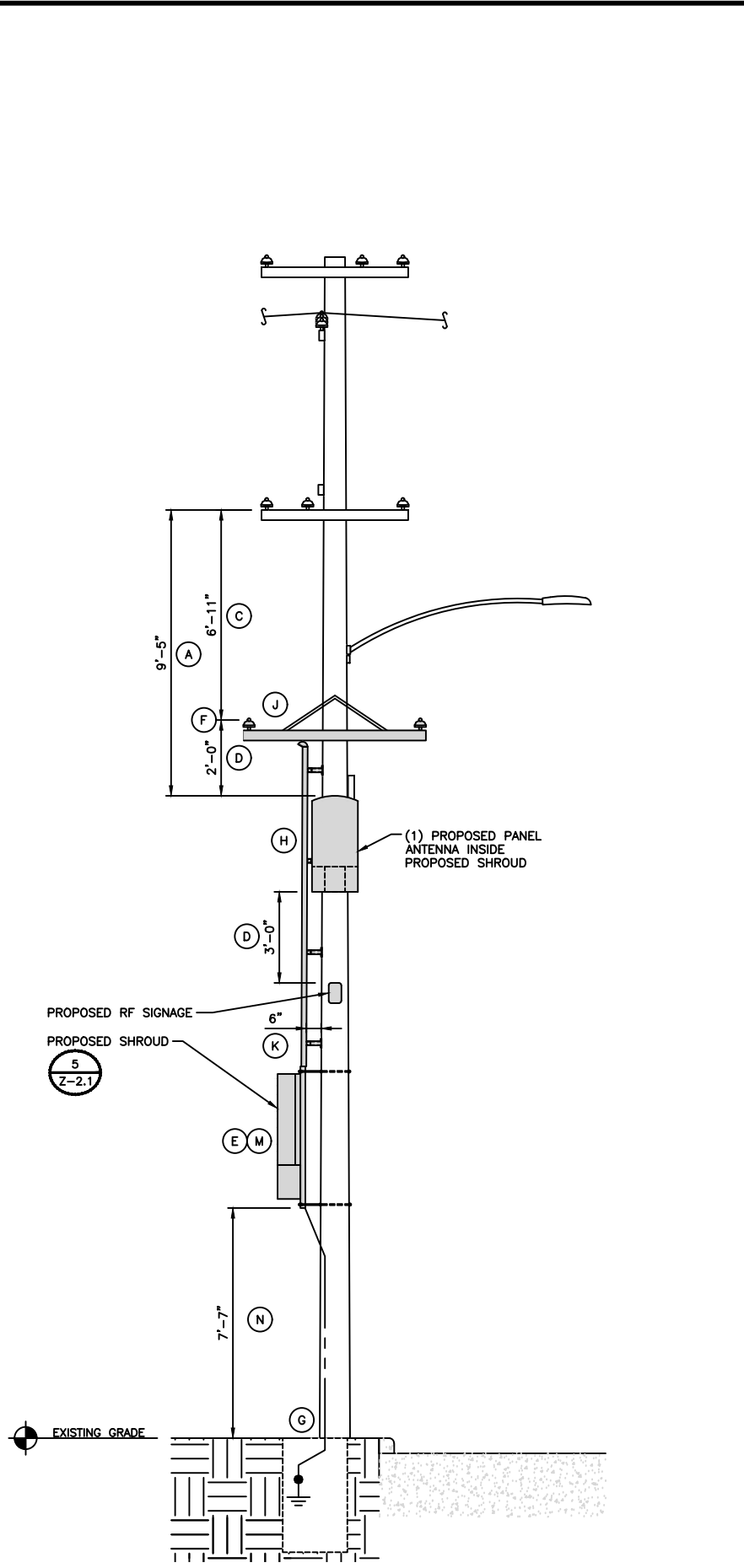
EQUIPMENT CLEARANCES
