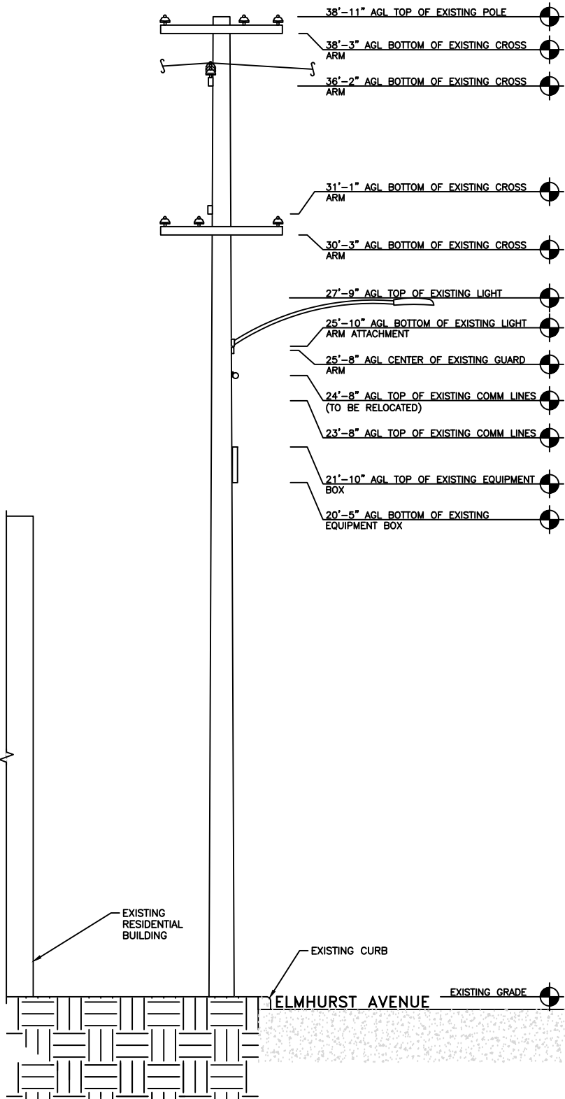
EXISTING WEST ELEVATION
