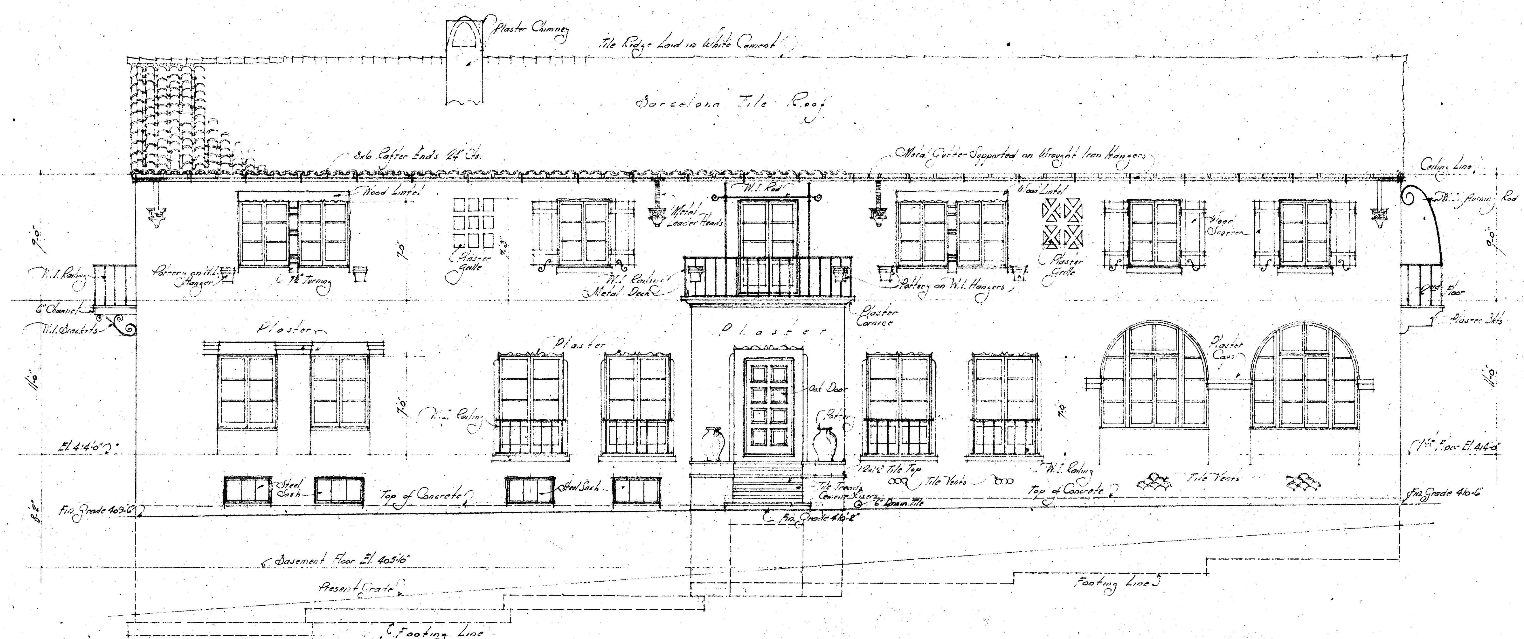
- SOUTH ELEVATION -
