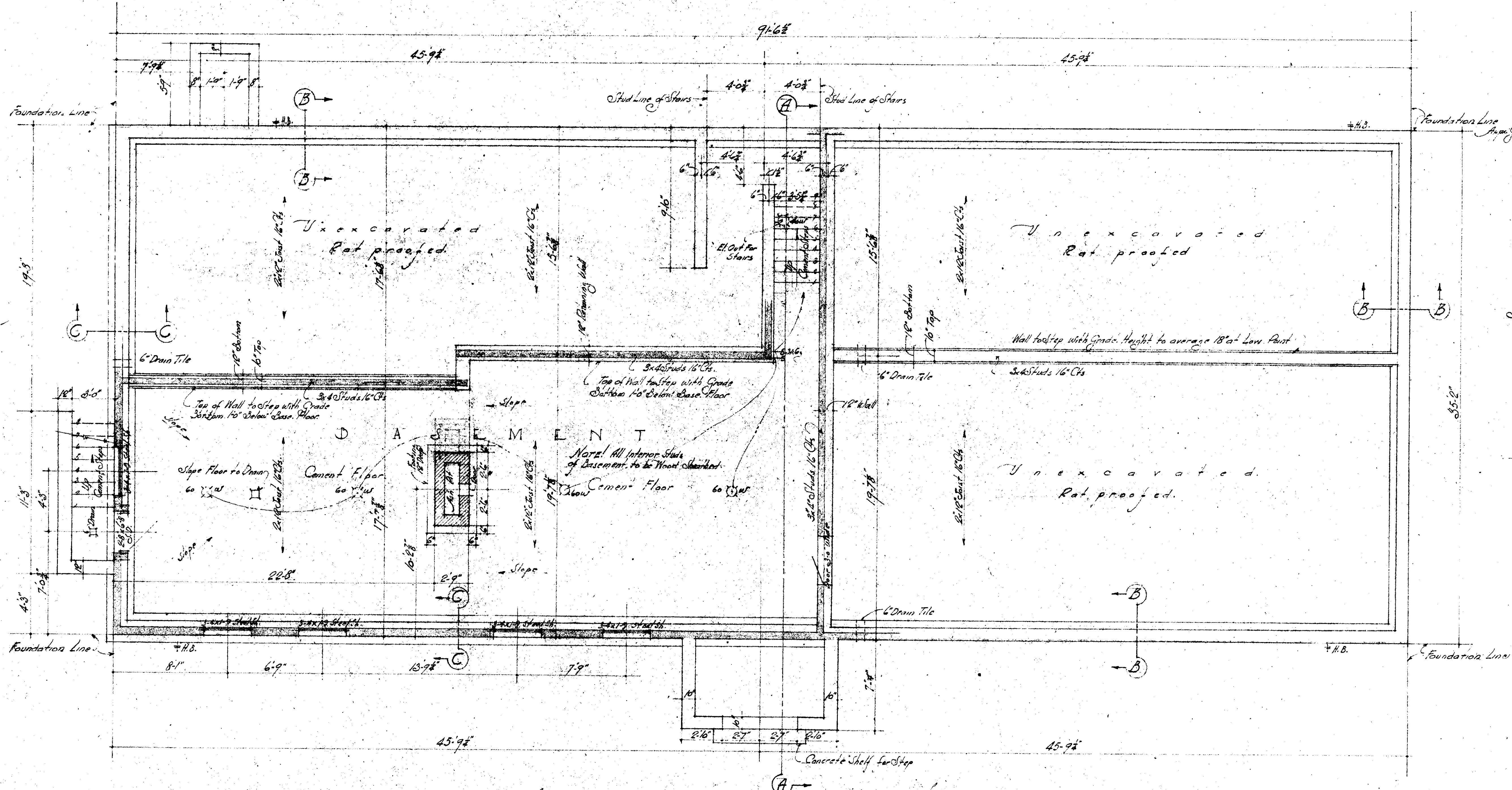
FOUNDATION PLAN
