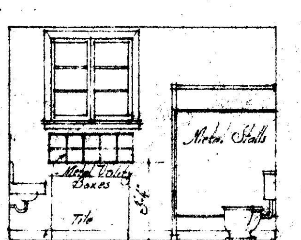
GIRLS' & BOYS' TOILET DETAILS
