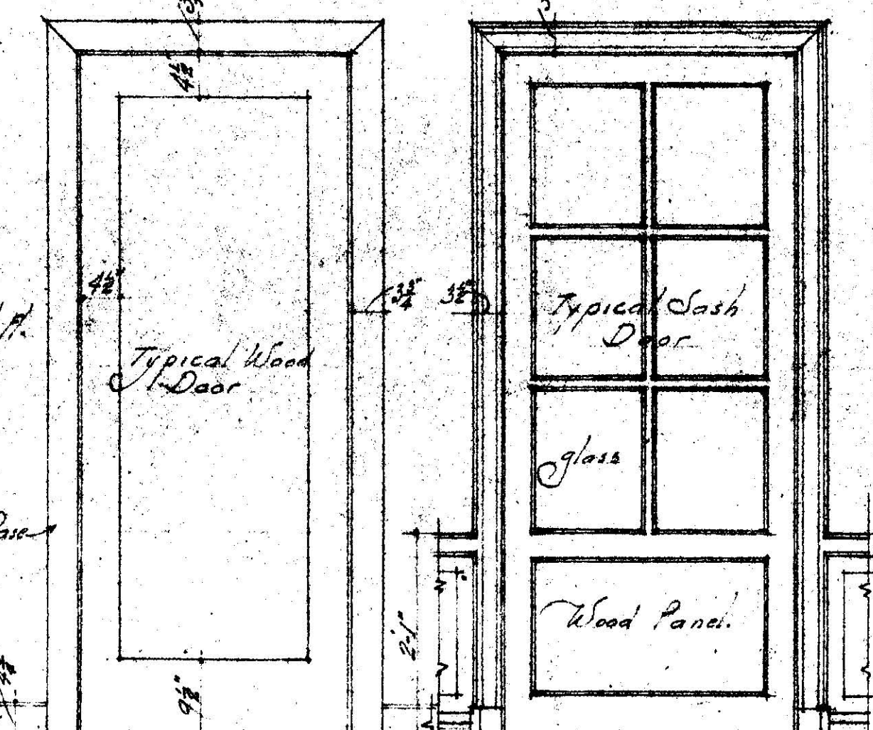
TYPICAL TRIM TRIM for L.R. DR. and STUDY Scale 1/4" = 1'-0"
