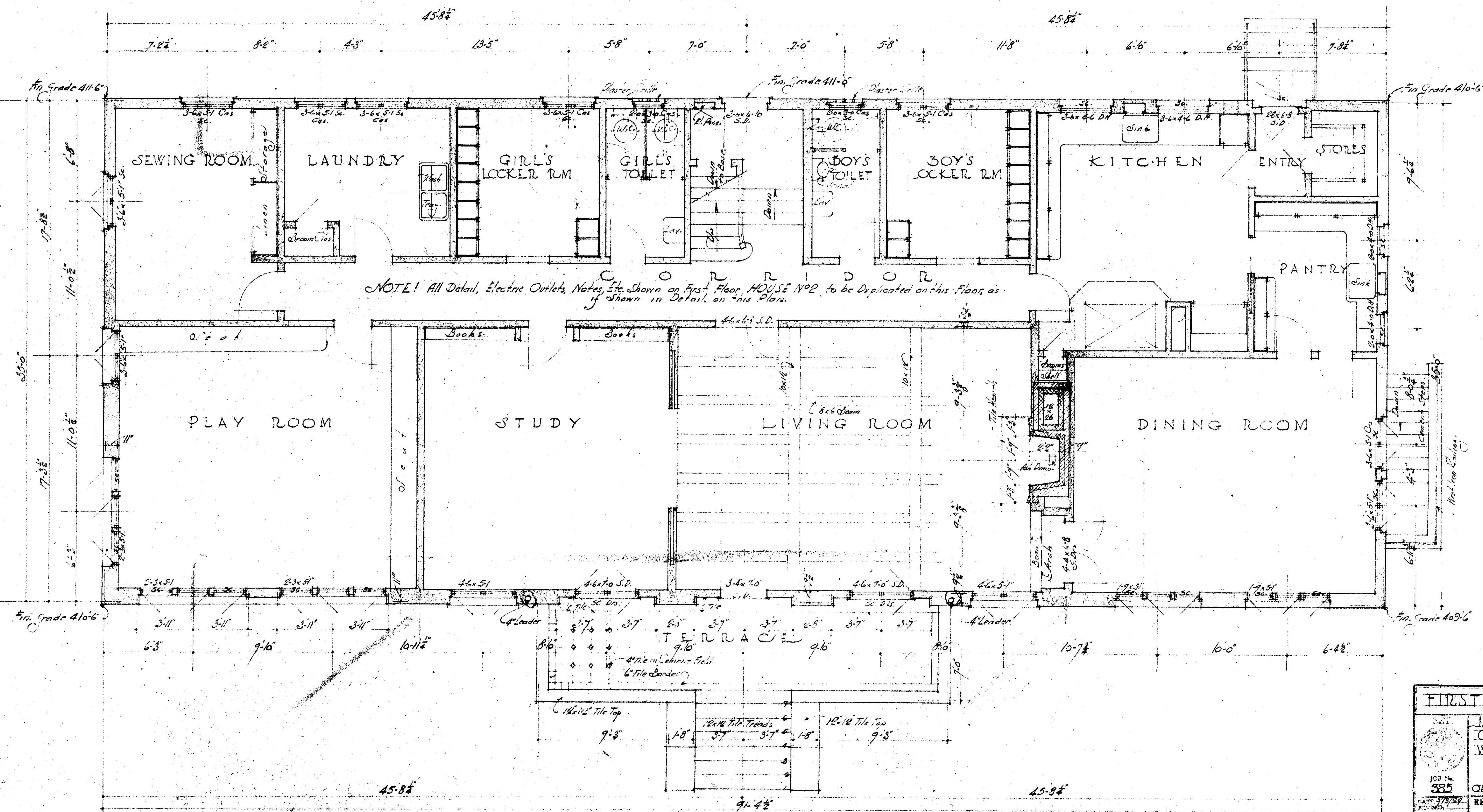
FIRST FLOOR
