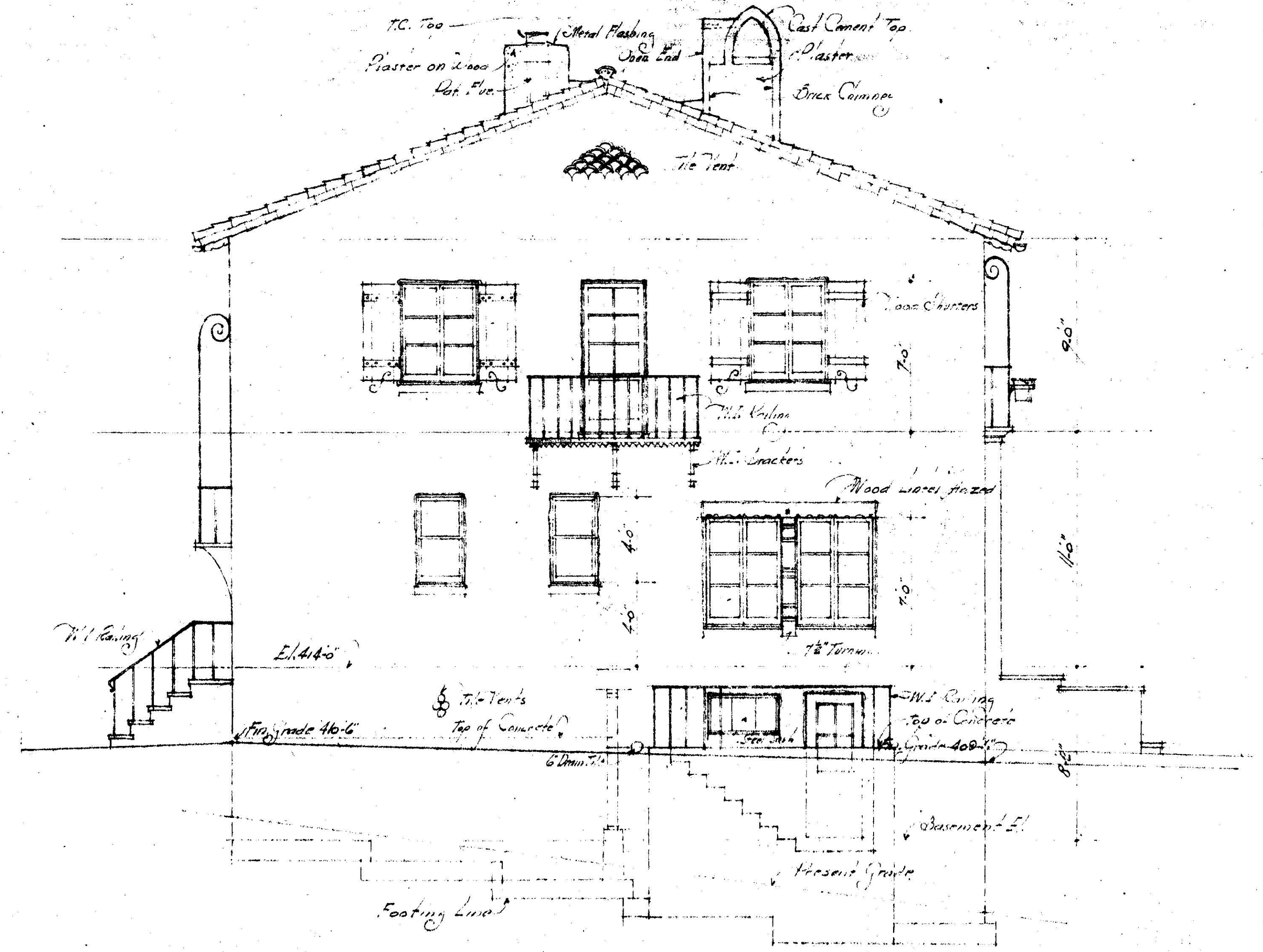
WEST ELEVATION
