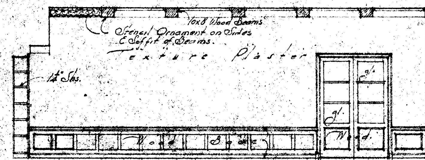
LIVING ROOM DETAILS
