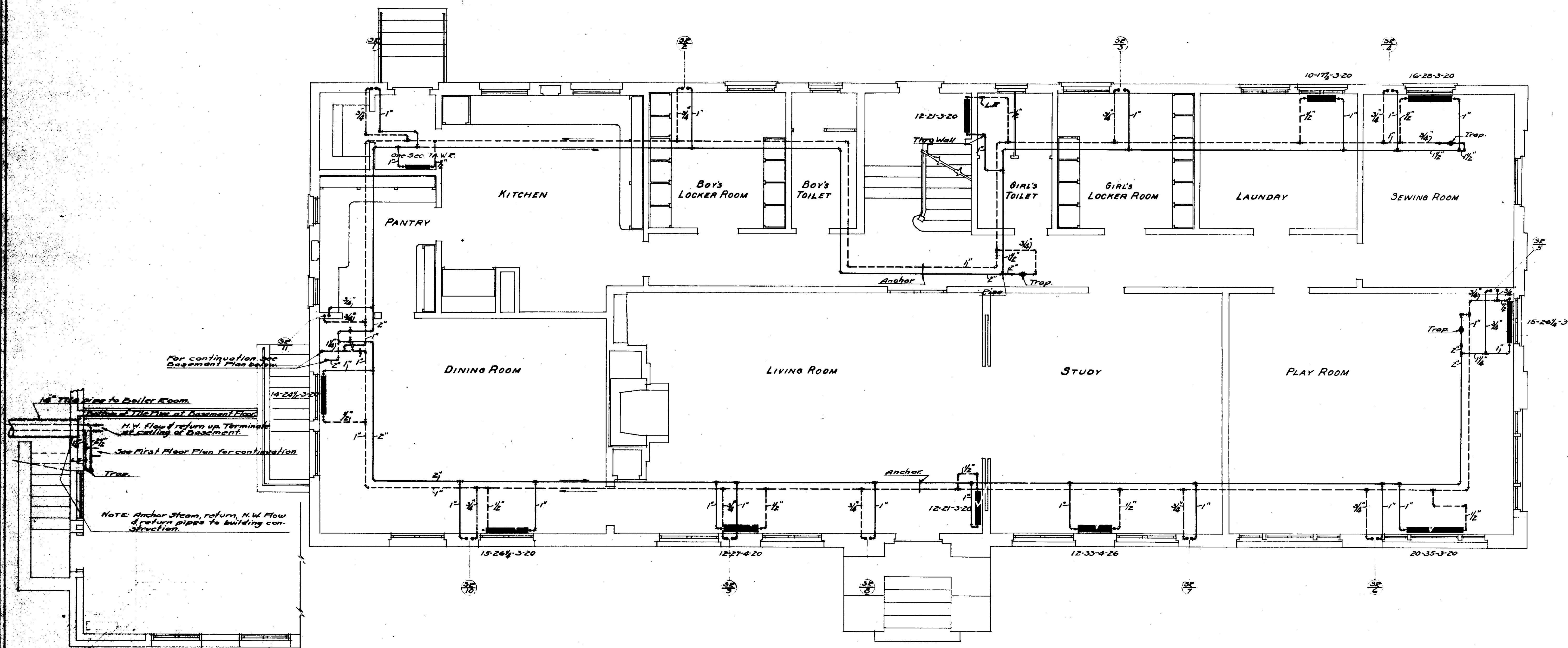
FIRST FLOOR PLAN Scale 1/4"=1'-0"
