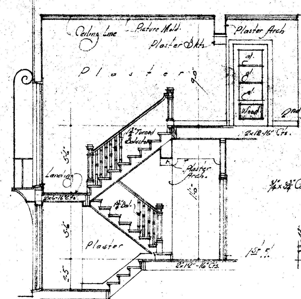
STAIR DETAIL
