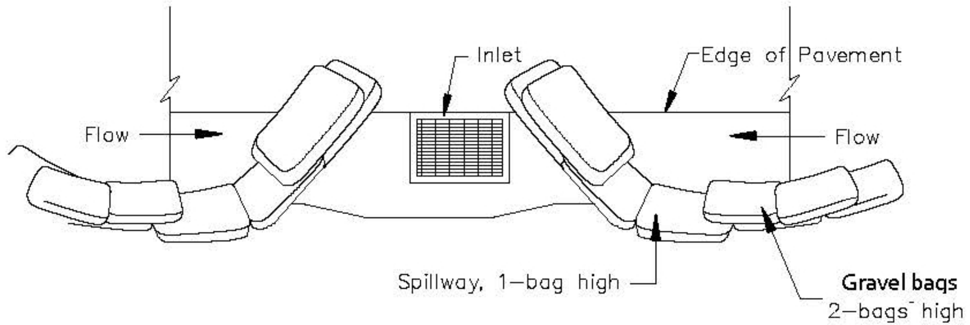
TYPICAL PROTECTION FOR INLET ON SUMP
