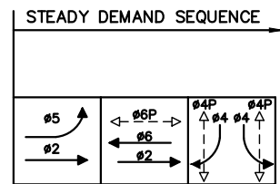
EXISTING PHASE DIAGRAM (TO REMAIN)
