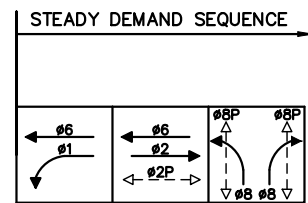
EXISTING PHASE DIAGRAM
